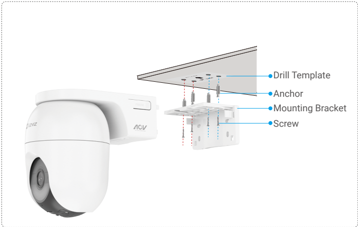
Fig. 1 Ceiling Mount
