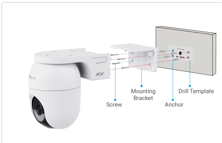
Fig. 2 Wall Mount
